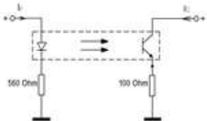
Test Circuit
